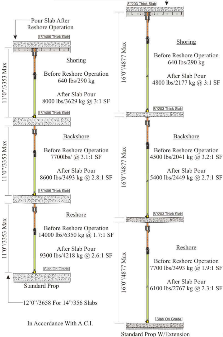
Prop Loads On Backprop & Reshore Prop For 8'x4'/2400x1200 Grid
